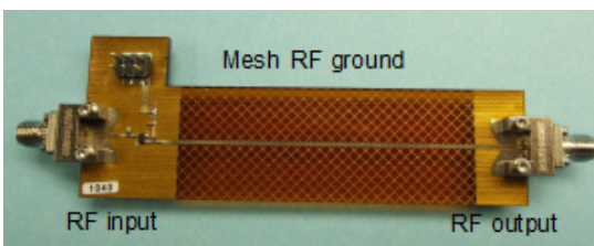
3D Printed RF Amplifier
